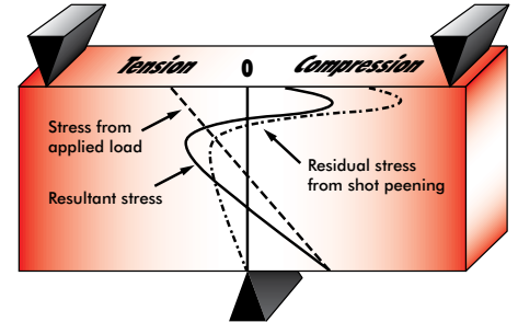
Shot peening influence on applied stress – algebraic reductions
